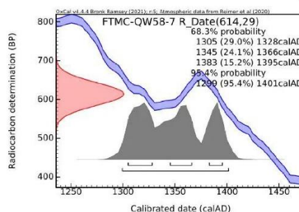
Fig. 1. Radiocarbon date 614±29BP (red), part of the calibration curve (blue) and the calibrated probability density function (grey) calculated in OxCal.
